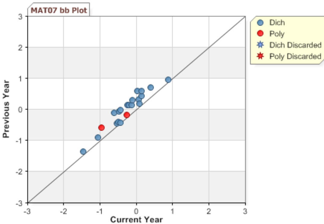
Figure K-24. 2011 MCAS: b -Plot—Mathematics Grade 7
