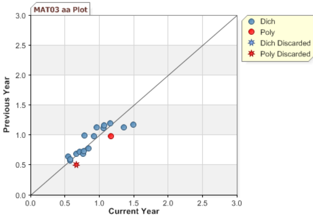
Figure K-15. 2011 MCAS: \alpha -Plot—Mathematics Grade 3
