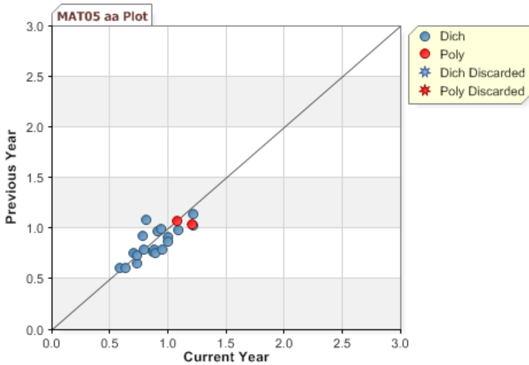
Figure K-19. 2011 MCAS: \alpha -Plot—Mathematics Grade 5
