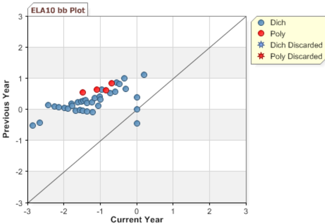
Figure K-14. 2011 MCAS: b -Plot—ELA Grade 10
