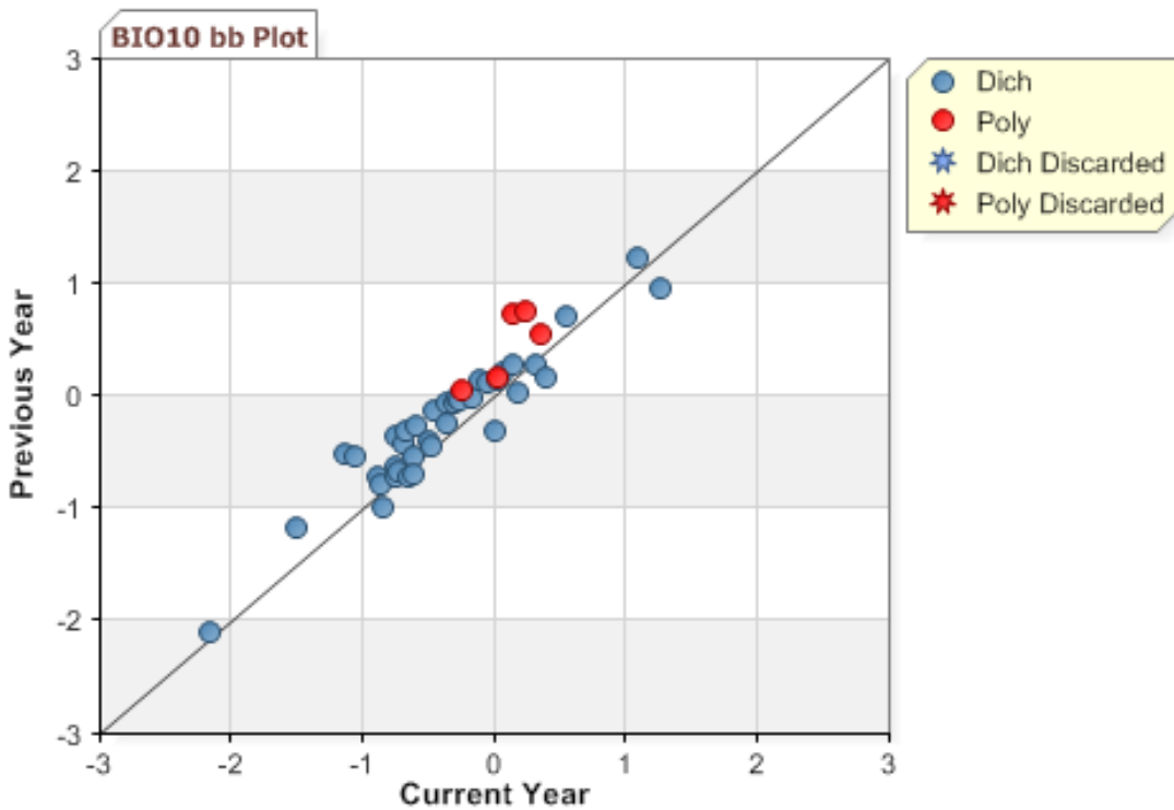
Figure K-34. 2011 MCAS: b -Plot—High School Biology
