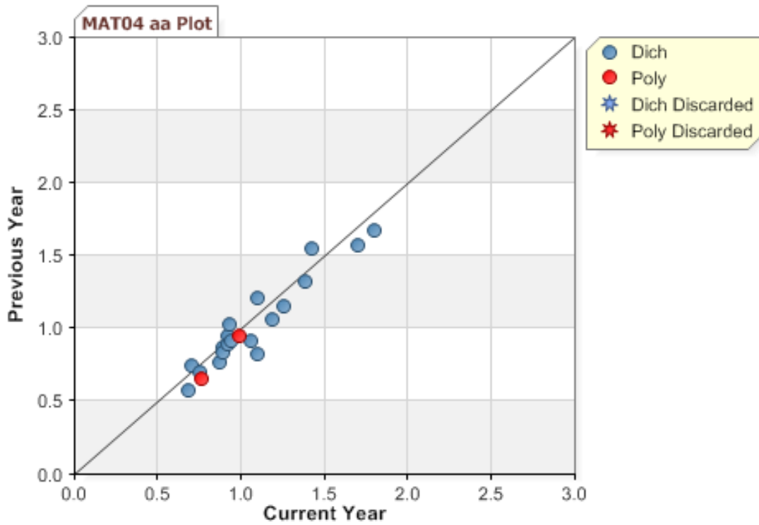
Figure K-17. 2011 MCAS: \alpha -Plot—Mathematics Grade 4
