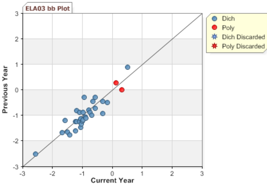
Figure K-2. 2011 MCAS: b -Plot—ELA Grade 3
