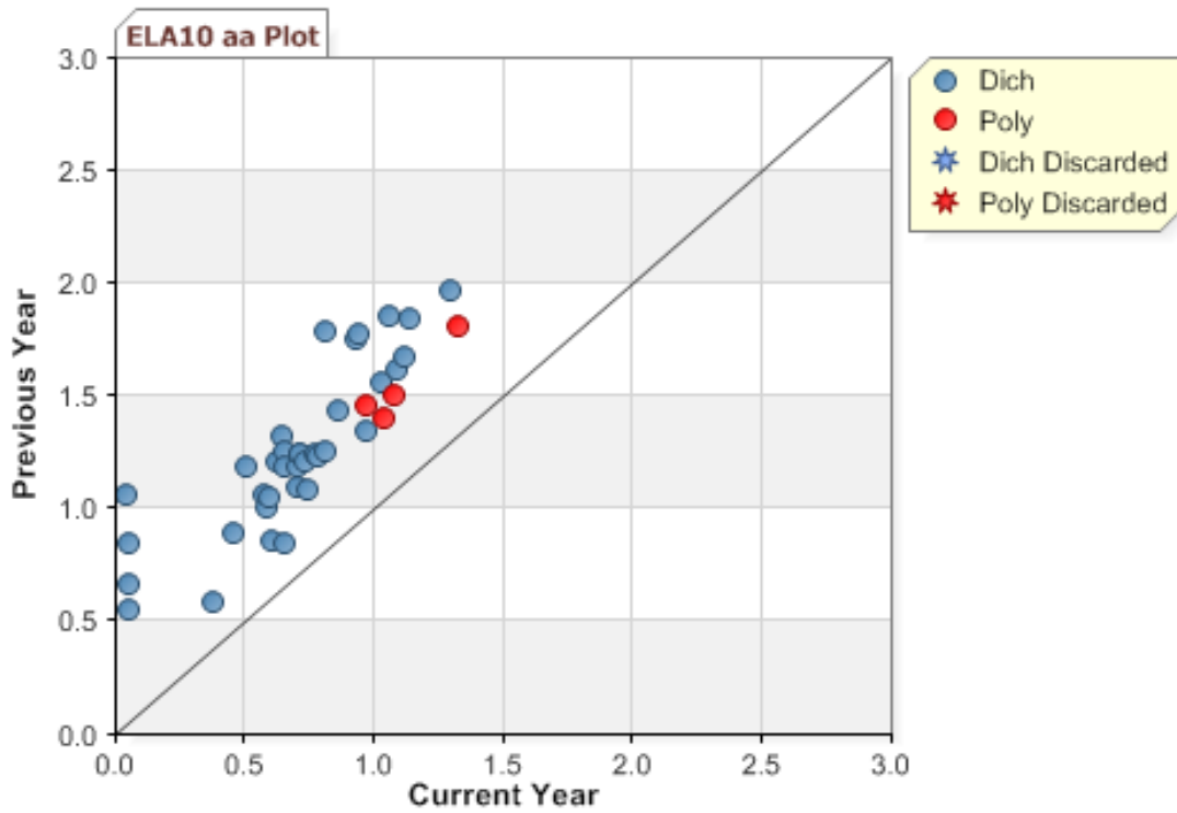
Figure K-13. 2011 MCAS: \alpha -Plot—ELA Grade 10
