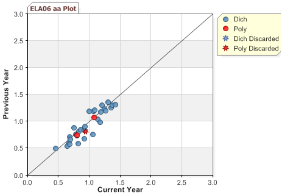
Figure K-7. 2011 MCAS: \alpha -Plot—ELA Grade 6
