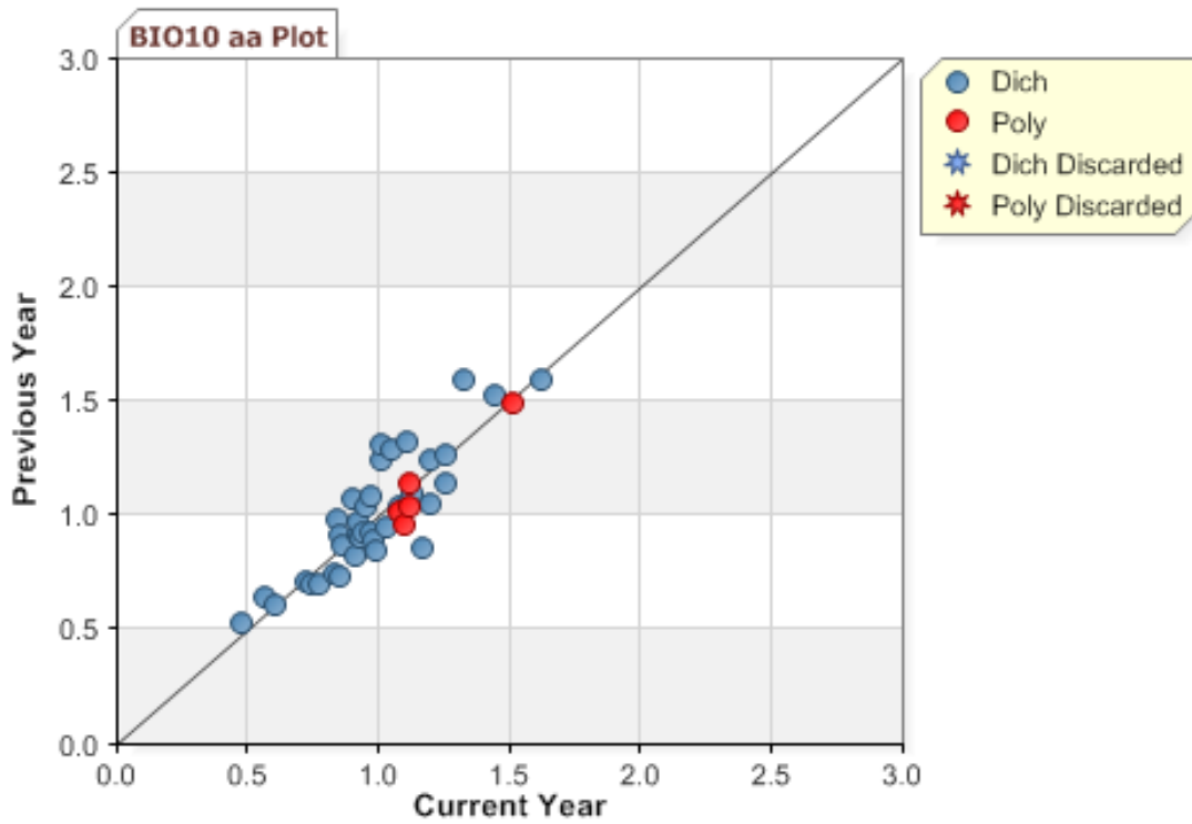
Figure K-33. 2011 MCAS: \alpha -Plot—High School Biology
