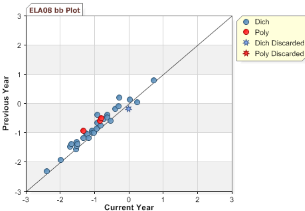
Figure K-12. 2011 MCAS: b -Plot—ELA Grade 8
