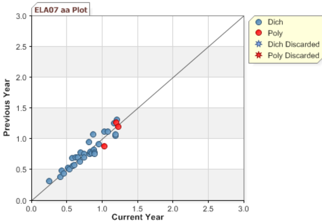
Figure K-9. 2011 MCAS: \alpha -Plot—ELA Grade 7
