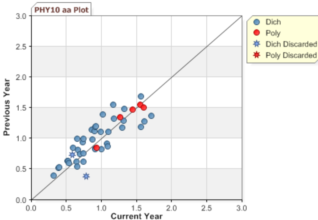
Figure K-37. 2011 MCAS: \alpha -Plot—High School Introductory Physics
