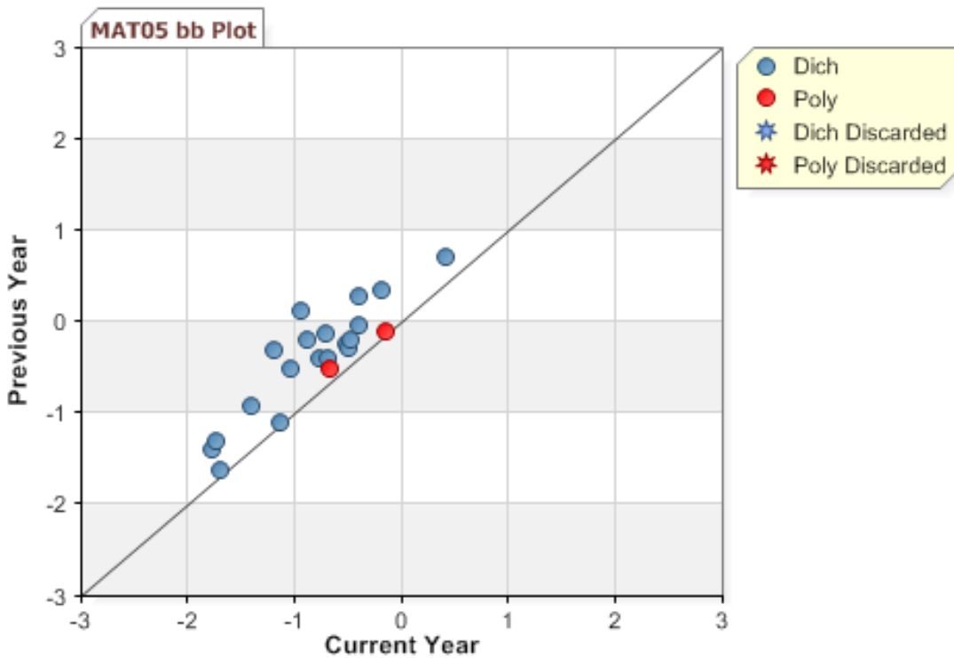
Figure K-20. 2011 MCAS: b -Plot—Mathematics Grade 5
