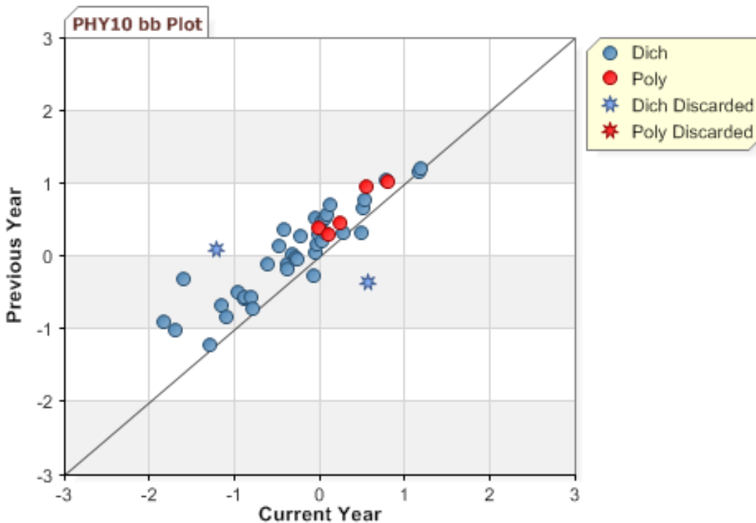
Figure K-38. 2011 MCAS: b -Plot—High School Introductory Physics
