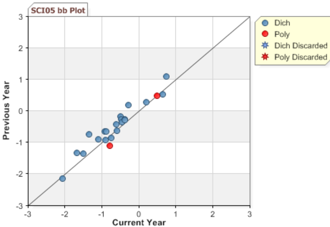
Figure K-30. 2011 MCAS: b -Plot—STE Grade 5
